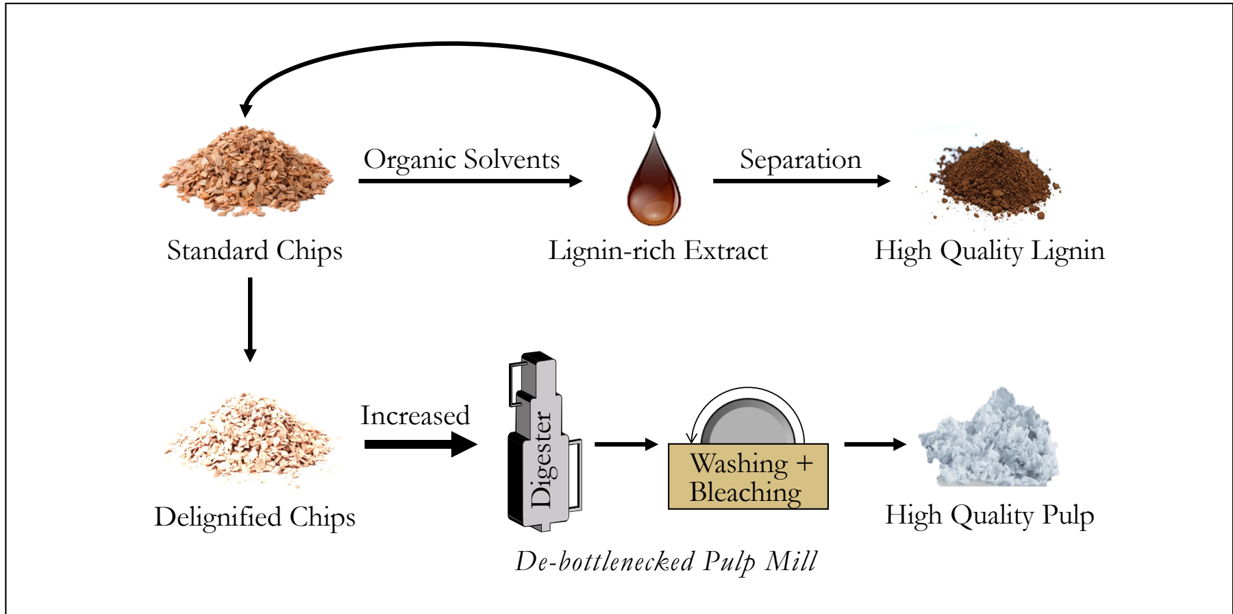
1. Lignin Value Prior to Pulping (LVPP): Organic solvent pretreatment increases pulp production and generates a new lignin stream.
